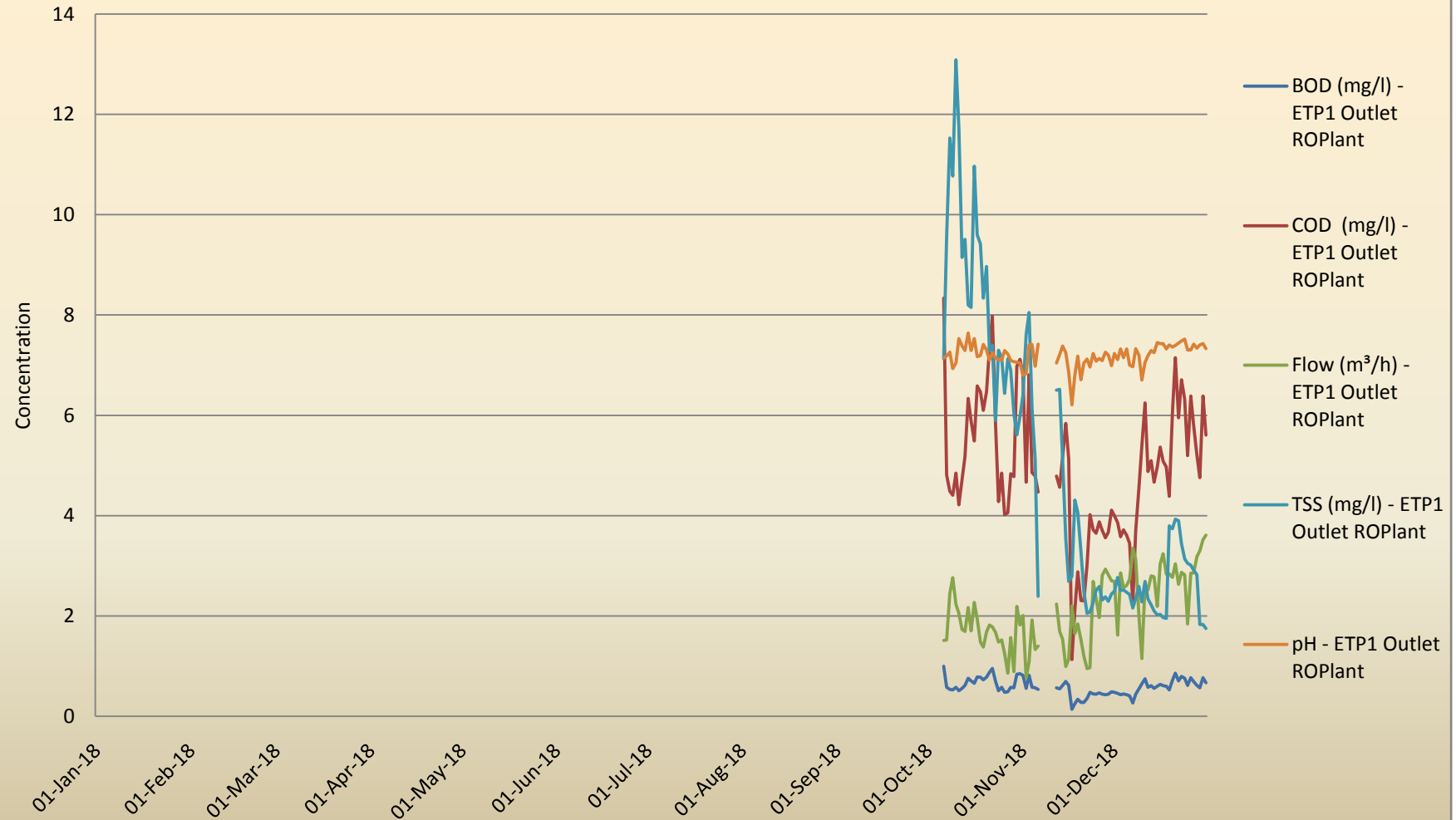
Annual Effluent Trend in M/s. Teva API India Ltd., Dist. Bhind (M.P.)
